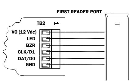
Reader Port 1 Typical D1/D0 or Clock/Data Reader
