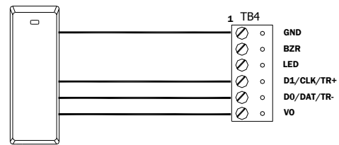
Typical RS-485 Device (OSDP Reader for Example)
